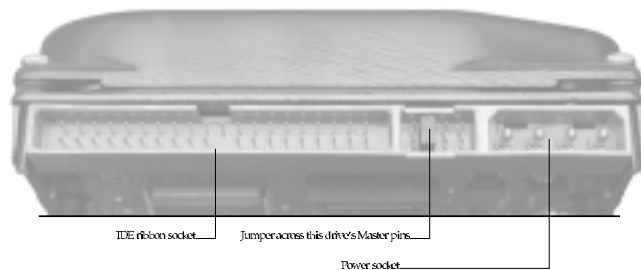
Figure 3.2 Connection end of a typical IDE drive
