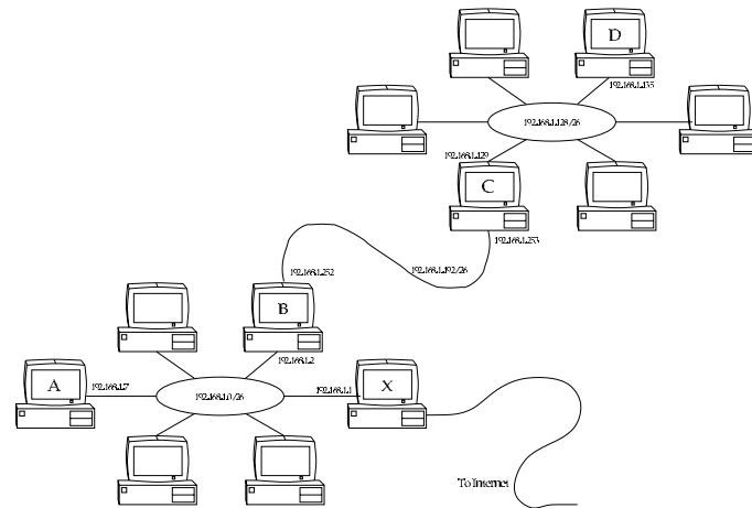
Figure 25.3 Two remotely connected networks
